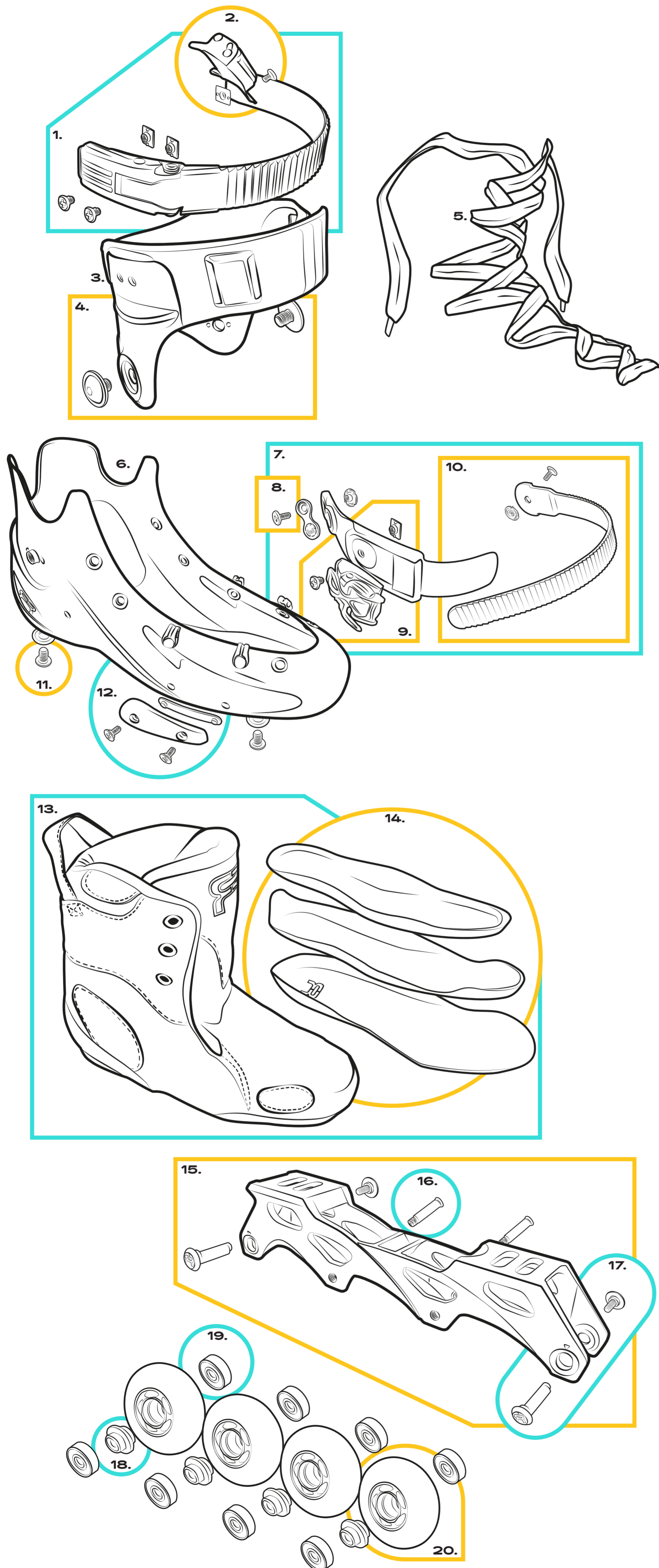
Exploded view - 2021 version
