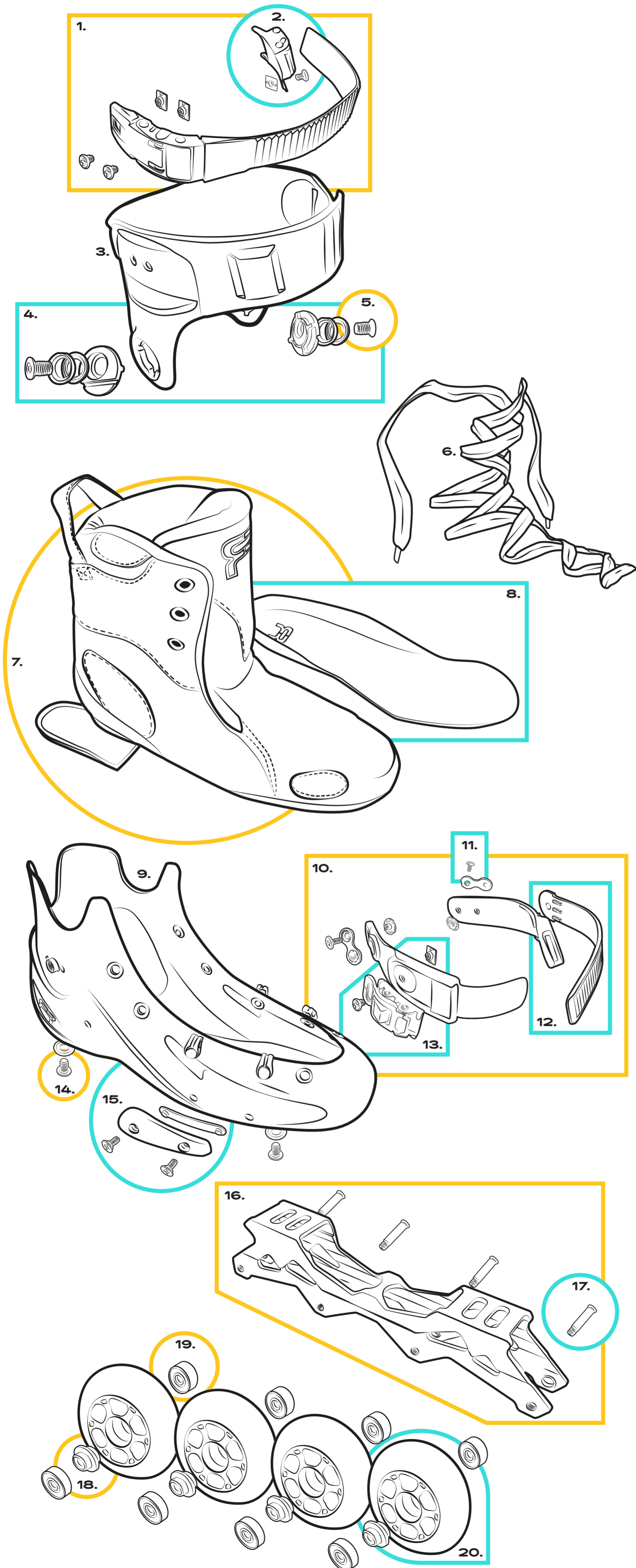
Exploded view - 2021 version
